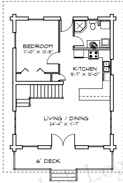
MAIN FLOOR 884 sq. ft.
