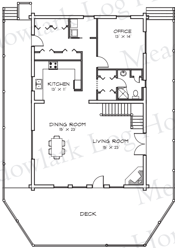
MAIN FLOOR 1536 sq. ft.
